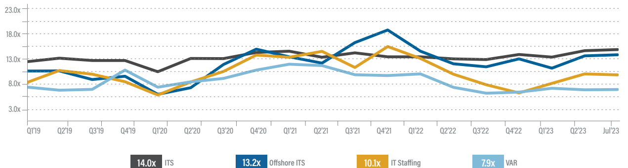
TEV / EBITDA
