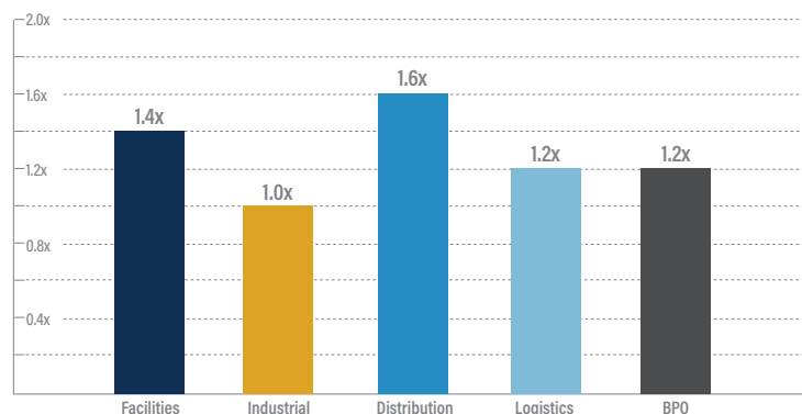
Enterprise Value / LTM Revenue
