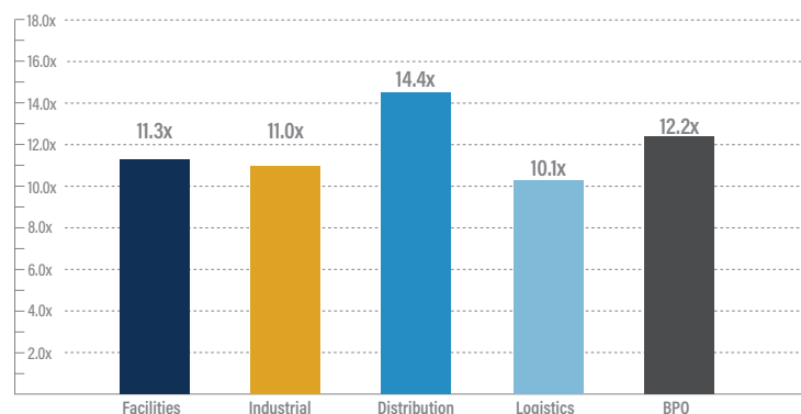
Enterprise Value / LTM EBITDA
