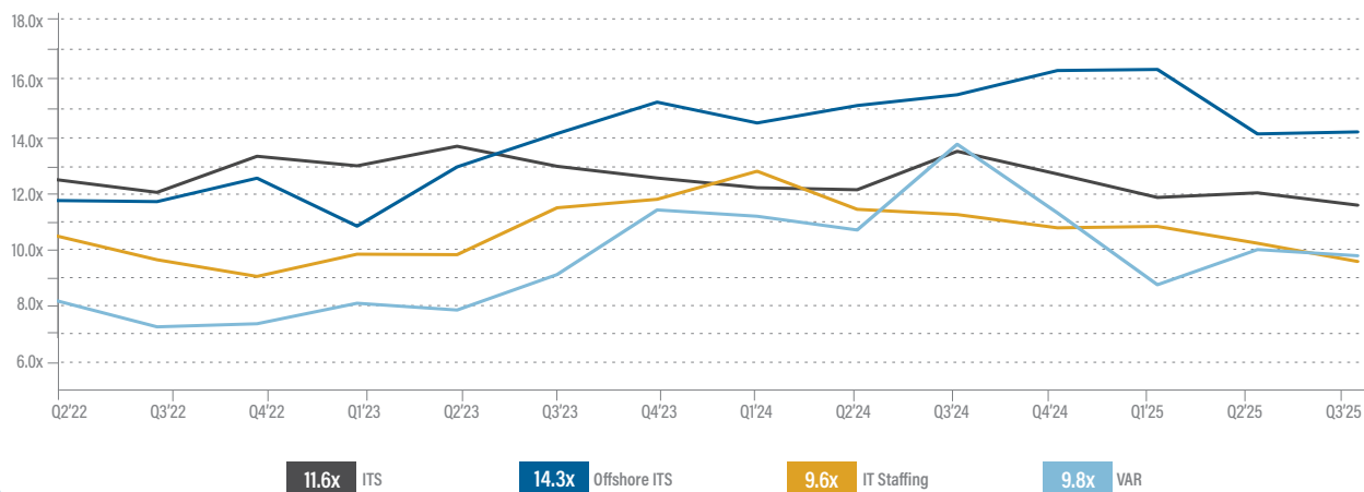
TEV / EBITDA
